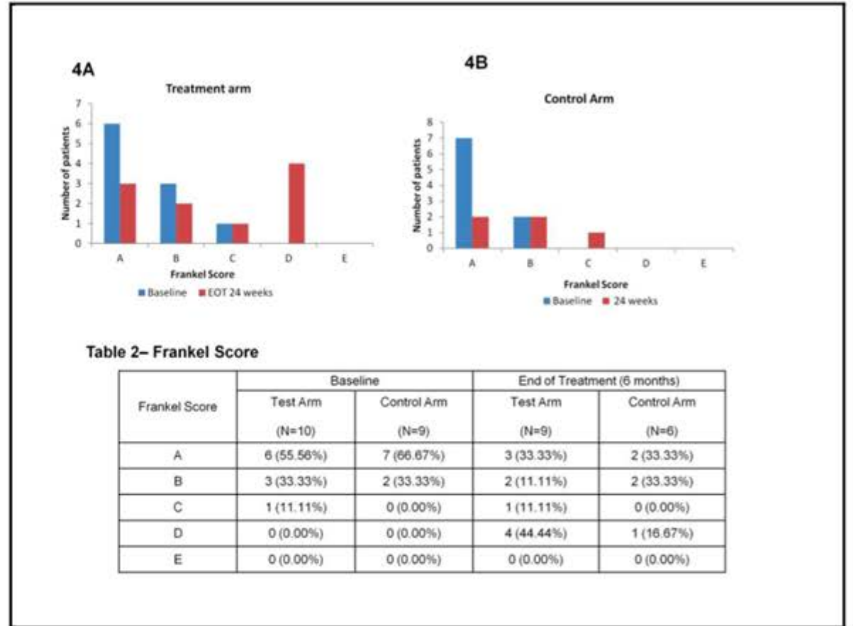
Figure 4: Frankel score
